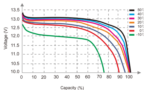
Different Temperature Discharge Curve(0.2C)
